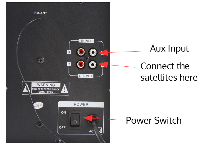
Back panel
